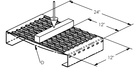
Deflection (D) is .56 inches with 500 lb. load
