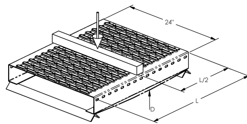
Concentrated Loading of Weight (Lbs.)
