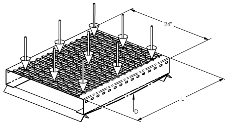
Uniform Loading of Weight (Lbs./Ft. 2 )
